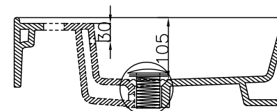
SECTION_VIEW A-A
