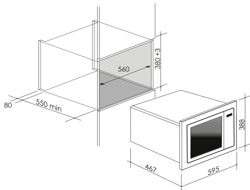
WALLMOUNT INSTALLATION
