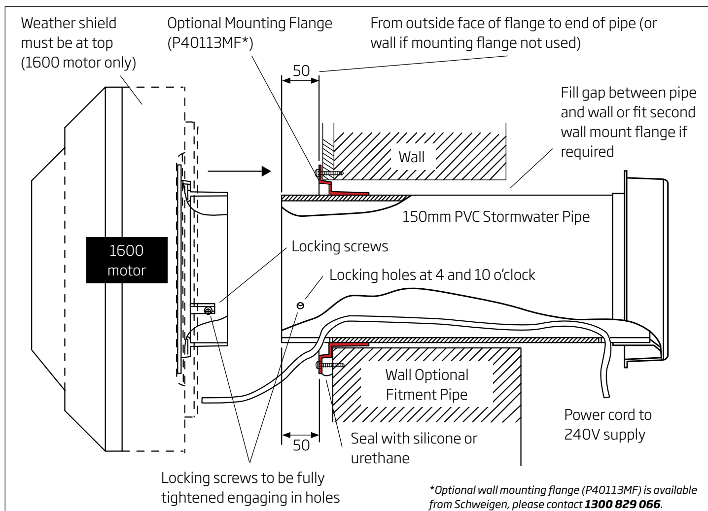
Figure 2 Wall Installation
