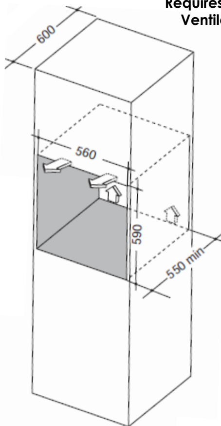
Base Installation Requires 30mm Ventilation
